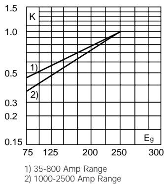
Fig. 1: 35-800 Amp Range
